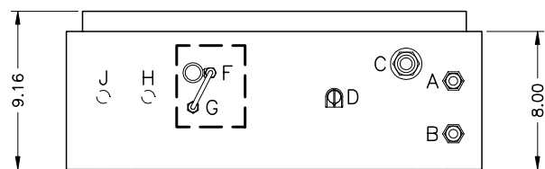
BOTTOM VIEW
