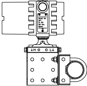
ANGLE MOUNT TO HORIZONTAL PIPE
