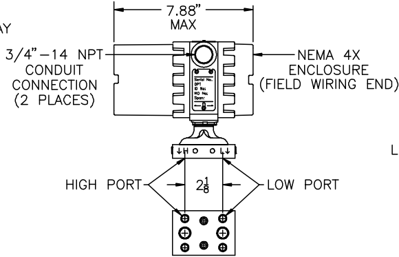
1/4"-18 NPT (FOR PRESSURE CONNECTIONS)
