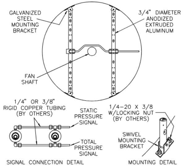
FOR INLETS 20" IN DIAMETER OR LARGER
