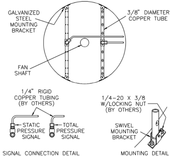
FOR INLETS LESS THAN 20" IN DIAMETER
